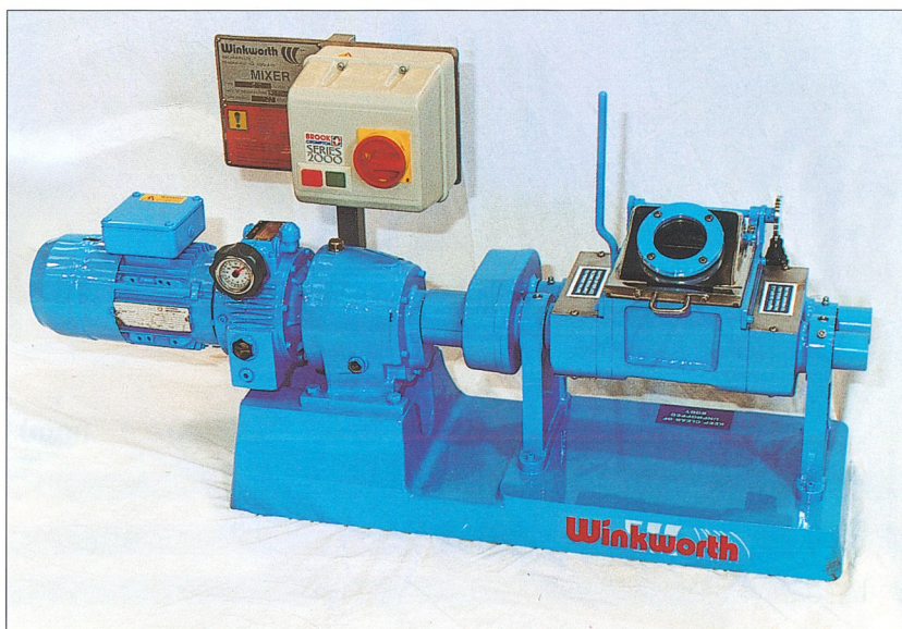
Model ZZ – 1.2 litre vacuum model with mechanical variable speed drive
